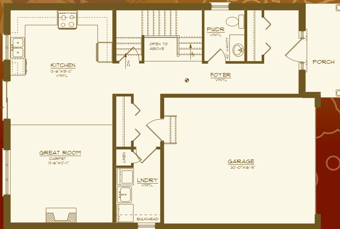
Main Floor 872 Sq. Ft.
